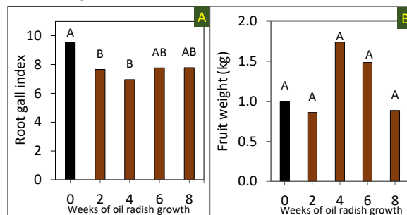
Fig. 3. Effect of oil radish growing time on A) pumpkin root gall index (1-10 scale) caused by root-knot nematodes, and B) pumpkin fruit weight per plot.
