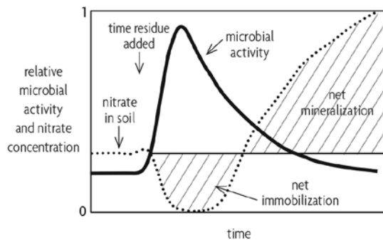
FIGURE 3.7. Changes in soil microbial activity and nitrate levels with the addition of plant residue with a low nitrogen content [12].
