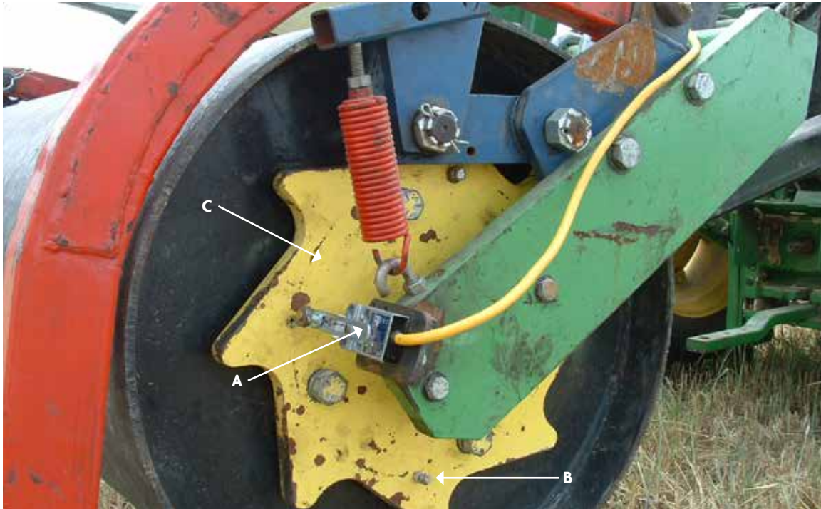
FIGURE 9.7. Side view of the smooth roller with crimping bar; (a) micro-switch, (b) engagement bolt with the switch's arm, and (c) eight-cam crimping bar control mechanism with clockwise rotation.
