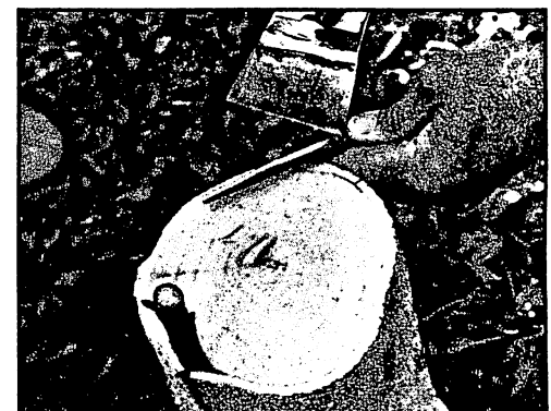
Fig. 25. One scion has been inserted, and the second is being tapered on the bark side with a chisel—a knife could be used instead.
