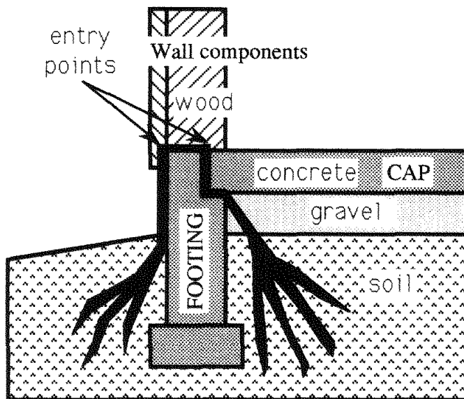
FLOATING SLAB
