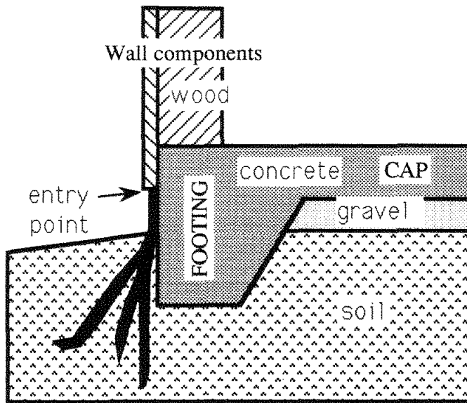
MONOLITHIC SLAB
